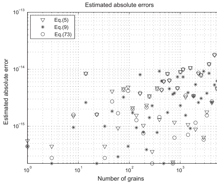
Fig. 14. Estimated absolute errors when computing q of (2) for honeycomb structures using the integral equations (5), (9) and (73). The grain conductivities vary between 0.1 and 10.
