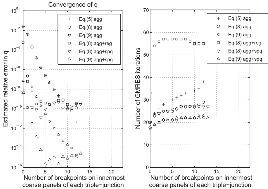
Fig. 7. Results for the Segmented Circle Problem with an aggressively graded mesh.
