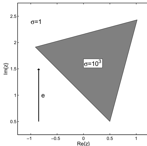
Fig. 2. The Triangle Problem.
