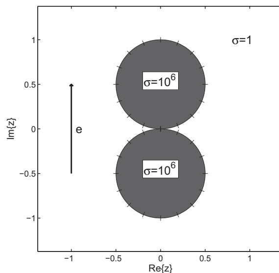
Fig. 8. Two conducting circles with radii R = 0.499999 separated by a distance of \delta = 0.000002 in a conducting plane. The panel placement on the coarse mesh is indicated. The reference solution is taken as q_{\text{ref}} = 5.1613733230816 .
