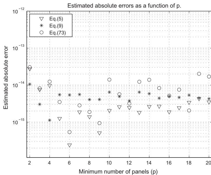
Fig. 13. Estimated absolute errors for q of (2) using the integral equation formulations (5), (9) and (73) with varying degree of overresolution. The inclusion consists of 390 grains. The reference value is taken as q_{ref} = -0.0326509925268292 .
