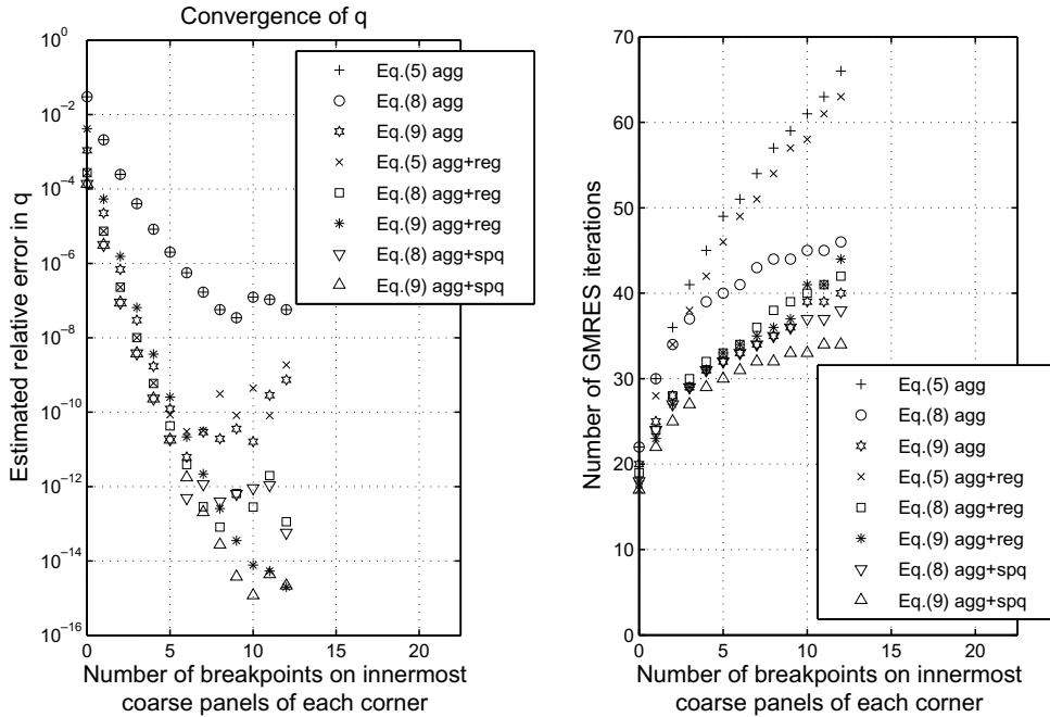
Fig. 4. Results for the Triangle Problem with an aggressively graded mesh. See Section 5 for the definition of breakpoints. The right image shows the number of GMRES iterations needed to reach a stopping criterion threshold of \epsilon_{mach} in the relative residual.
