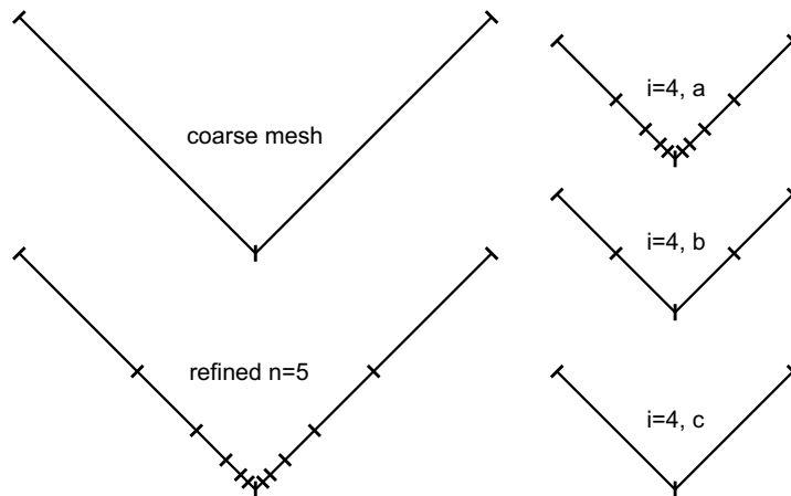
Fig. 1. Placement of panels on \Gamma_1 of a corner in the shape of a wedge. Upper left: Panels of the coarse mesh on \Gamma_1 . Lower left: Panels of a n -ply refined mesh on \Gamma_1, n = 5 . Right: Panels on \Gamma_{ii} upon which the grids \mathcal{G}_{ia}, \mathcal{G}_{ib} , and \mathcal{G}_{ic} are constructed for i = 4 and n = 5 . Note that \mathcal{G}_{ia} and \mathcal{G}_{ib} coincide for i = 1 .
