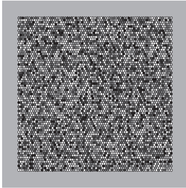
Fig. 12. A perturbed honeycomb structure consisting of 5293 grains. The conductivity varies between \sigma = 0.1 (light) and \sigma = 10 (dark). The background material has conductivity \sigma_0 = 1 . There are 10,878 corners and triple-junctions in the structure.
