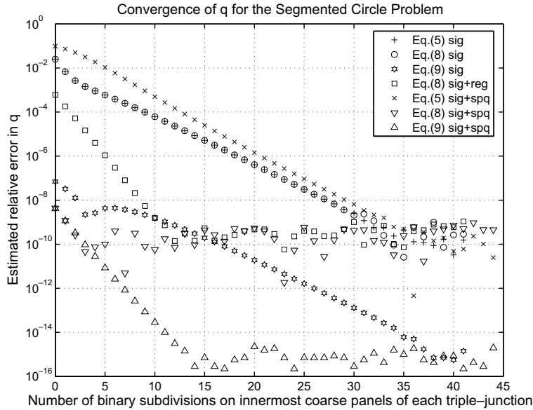
Fig. 6. Results for the Segmented Circle Problem with a simply graded mesh. The reference solution is taken as q_{ref} = 6.25303717710058 .
