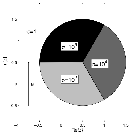
Fig. 5. The Segmented Circle Problem.
