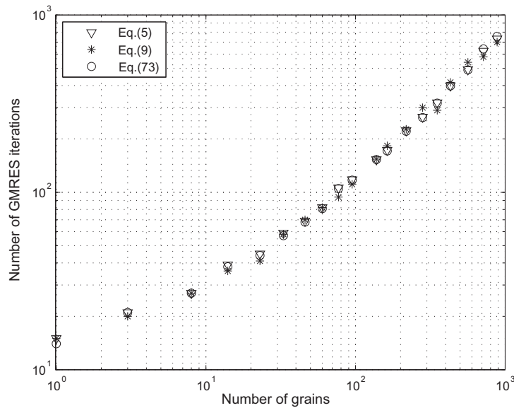
Fig. 16. Same as in Fig. 15, but the grain conductivities vary between 10^{-3} and 10^3 .
