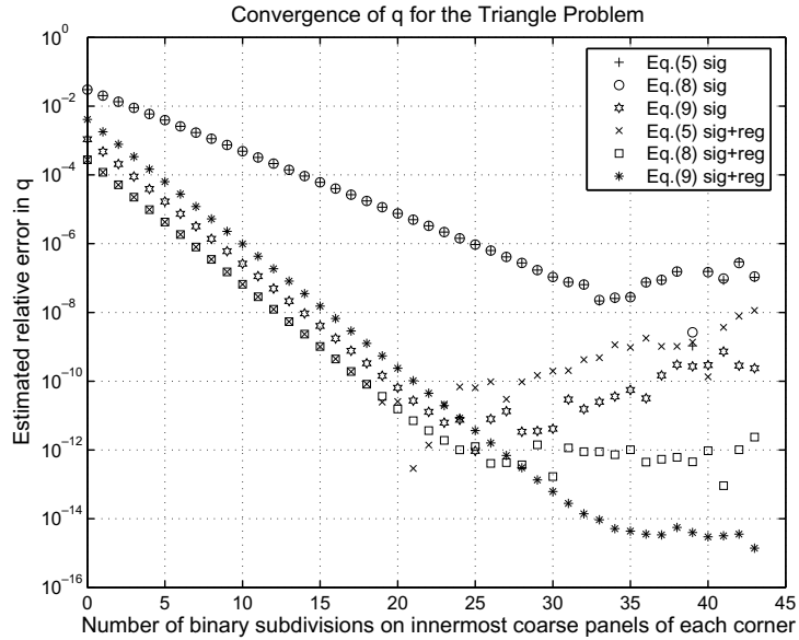
Fig. 3. Results for the Triangle Problem with a simply graded mesh. The reference solution is taken as q_{ref} = 4.455790323135370 .
